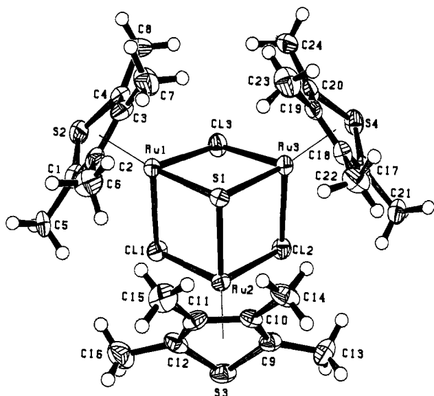
Figure 4. Structure of the cation in [(TMT)RuCl] 3 S(PF 6 ).
