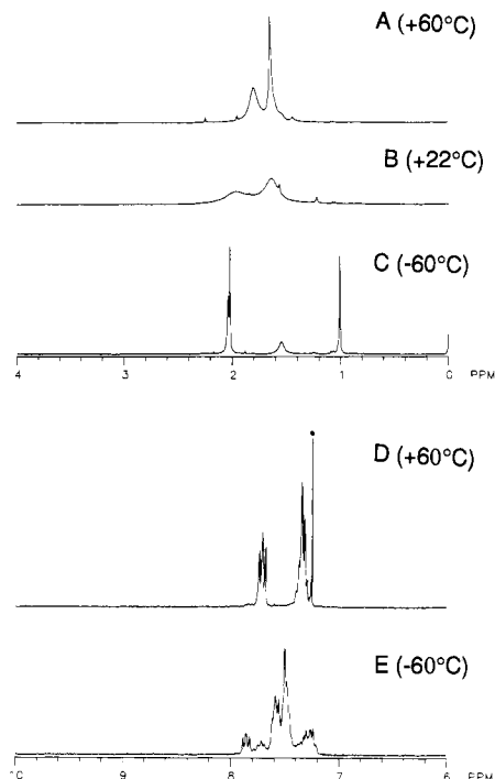
Figure 3. 300-MHz ^1H NMR spectra of CD_2Cl_2 solutions of (TMT)RuCl_2(PPh_3) in the methyl (A–C) and phenyl regions (D–E). Small peaks at 2.25 and 1.96 ppm in A are due to a trace of free TMT.
